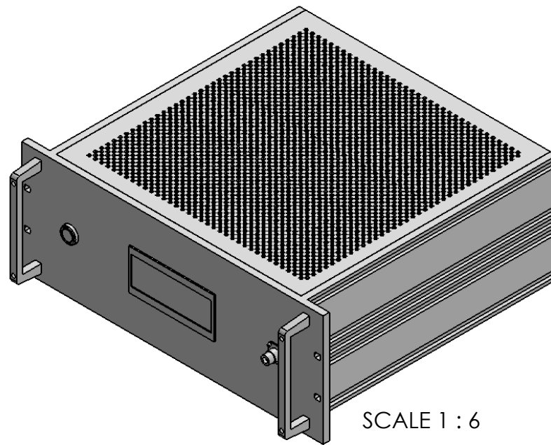
Power Amplifier Rack 3D
